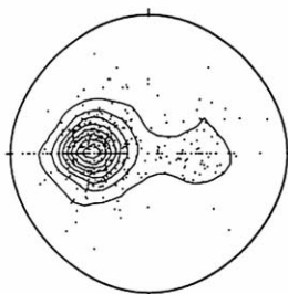
poles to magmatic foliation
