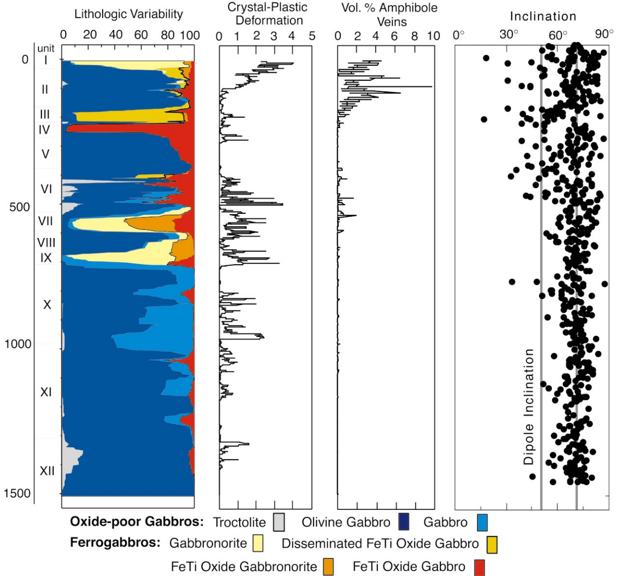
Fig. 1. Hole 735B lithostratigraphic variations [3,4]. Left: Relative abundances of igneous rocks averaged over a moving 20 m interval. Rock names follow the standard IUGS classification with modifiers to indicate oxide abundance. Middle left: Crystal-plastic deformation intensity from zero (undeformed) to five (ultramylonite). Middle right: Amphibole veins by core percentage averaged over a 2 m window. Right: Characteristic remanent inclinations. Mean inclination value (right gray line) is based on the inclination only averaging technique of McFadden and Reid [5].
