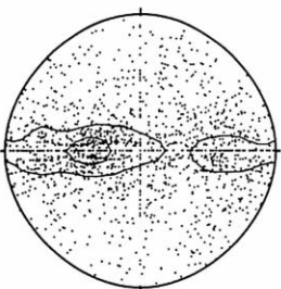
poles to veins
