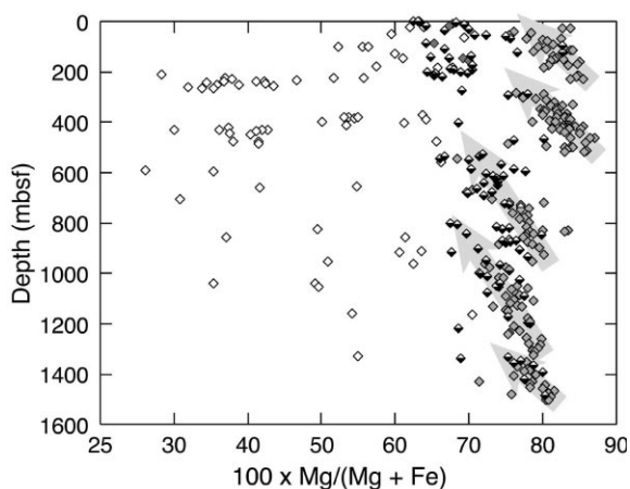
Fig. 2. Shipboard XRF whole rock gabbro molecular Mg/(Mg+Fe^{2+}) with FeO=0.85 \times Fe_2O_3 [3,4]. Filled symbols: TiO_2 < 0.4 wt%, half-filled symbols: TiO_2 from 0.4 to 1.0 wt%, and open symbols: TiO_2 > 1.0 wt%.
