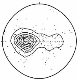
poles to crystal-plastic foliation
