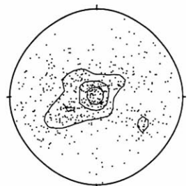
poles to faults
